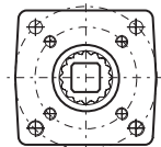
Insert mounting acc. ISO 5211
