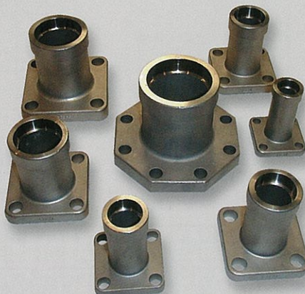
Complete Range of Extended Socket Weld Tailpieces
